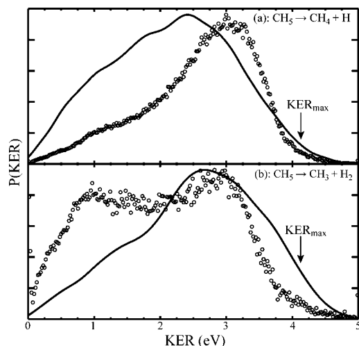
Figure 2. (a) P(\text{KER}) distribution for \text{CH}_5^+ \rightarrow \text{CH}_4 + \text{H} and (b) \text{CH}_5^+ \rightarrow \text{CH}_3 + \text{H}_2 . The open circles represent the experimental KER, while the solid line is the theoretical KER, with \text{KER}_{\text{max}} noted.
